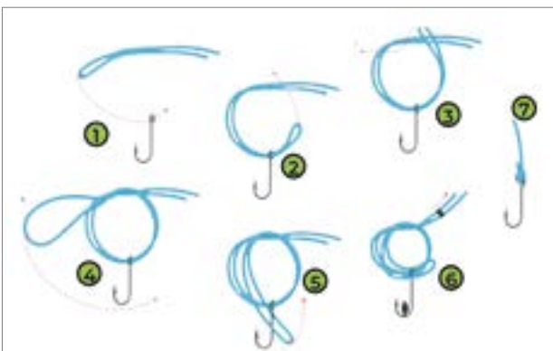
SINGLE PALOMAR KNOT
