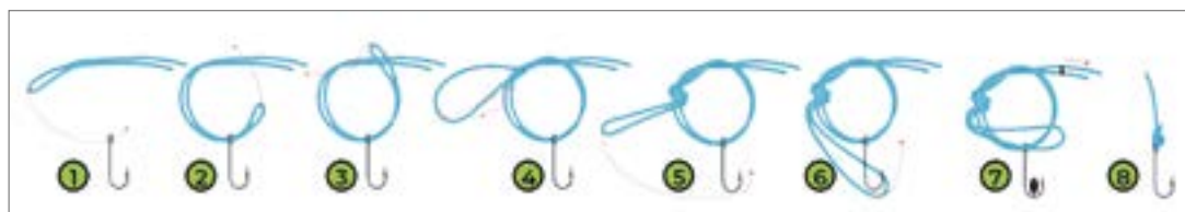
DOUBLE PALOMAR KNOT
